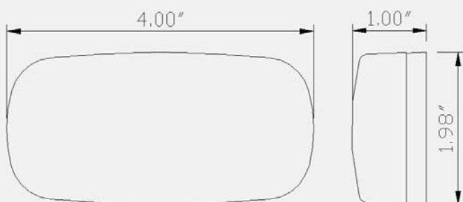
Clearance marker light w/ reflex lens
